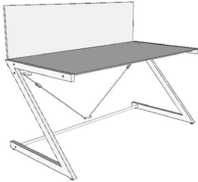
DESK WALL FROM Z-LINE/DD Z-LINE SERIES
